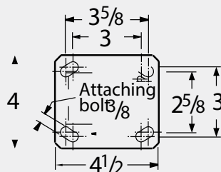
Top Plate Dimensions
